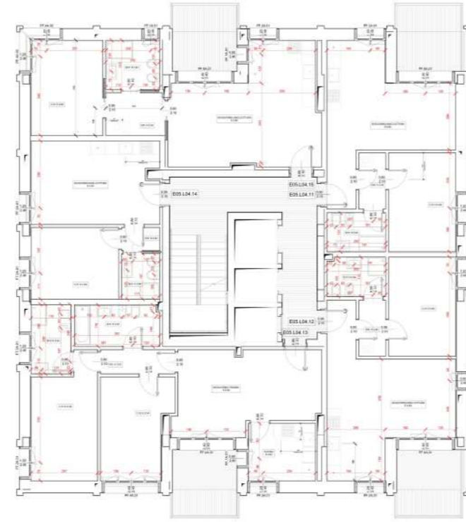
LEVEL 4 PLAN - WINDOWS & PLUMBING FIXTURES
