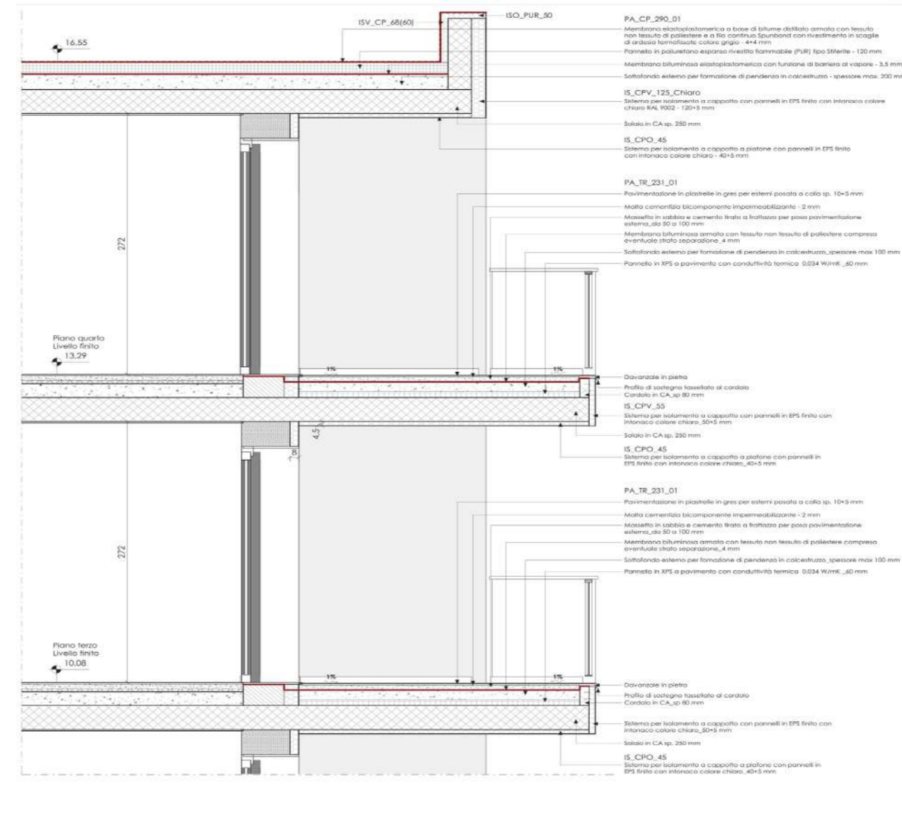
WALL SECTION: ROOF & TERRACE COMPOSITION
