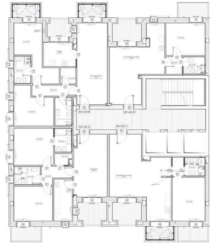
LEVEL 4 PLAN
