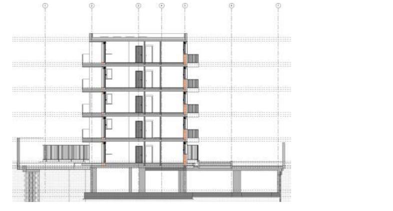
SECTION 02
